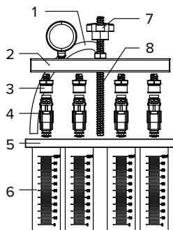
(Top-in fuel injector installation diagram)
